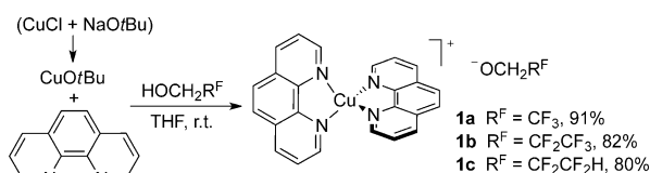
Scheme 2. Synthesis of copper(I) fluoroalkoxide complexes 1a–c . r.t. = room temperature.
